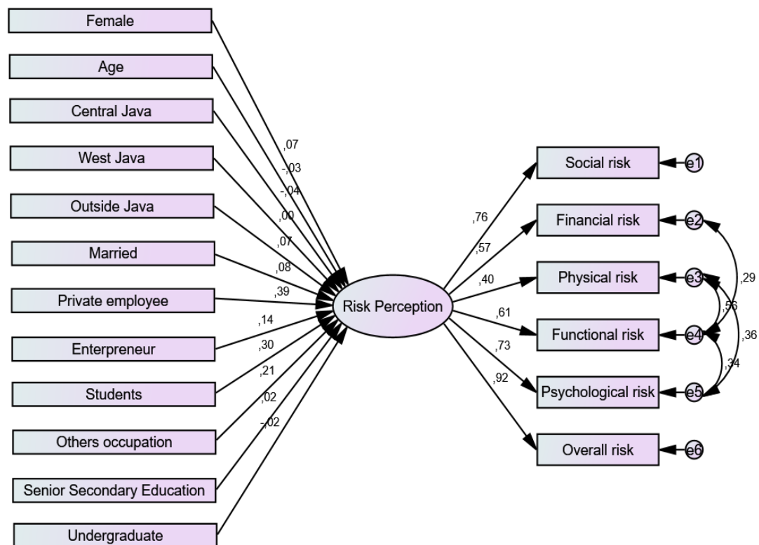
Figure 1. Multiple Indicator Multiple Cause (MIMIC) model showing the impact of covariate variable on the risk perception as latent variable
